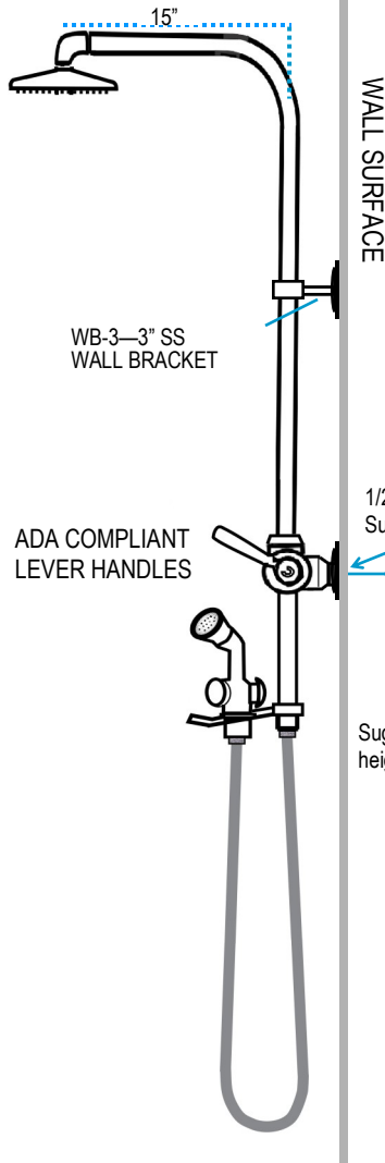
FRONT VIEW
